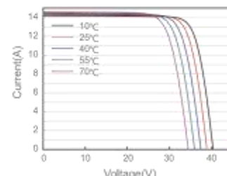
Current-Voltage Curve JAM54D41-440/LB
